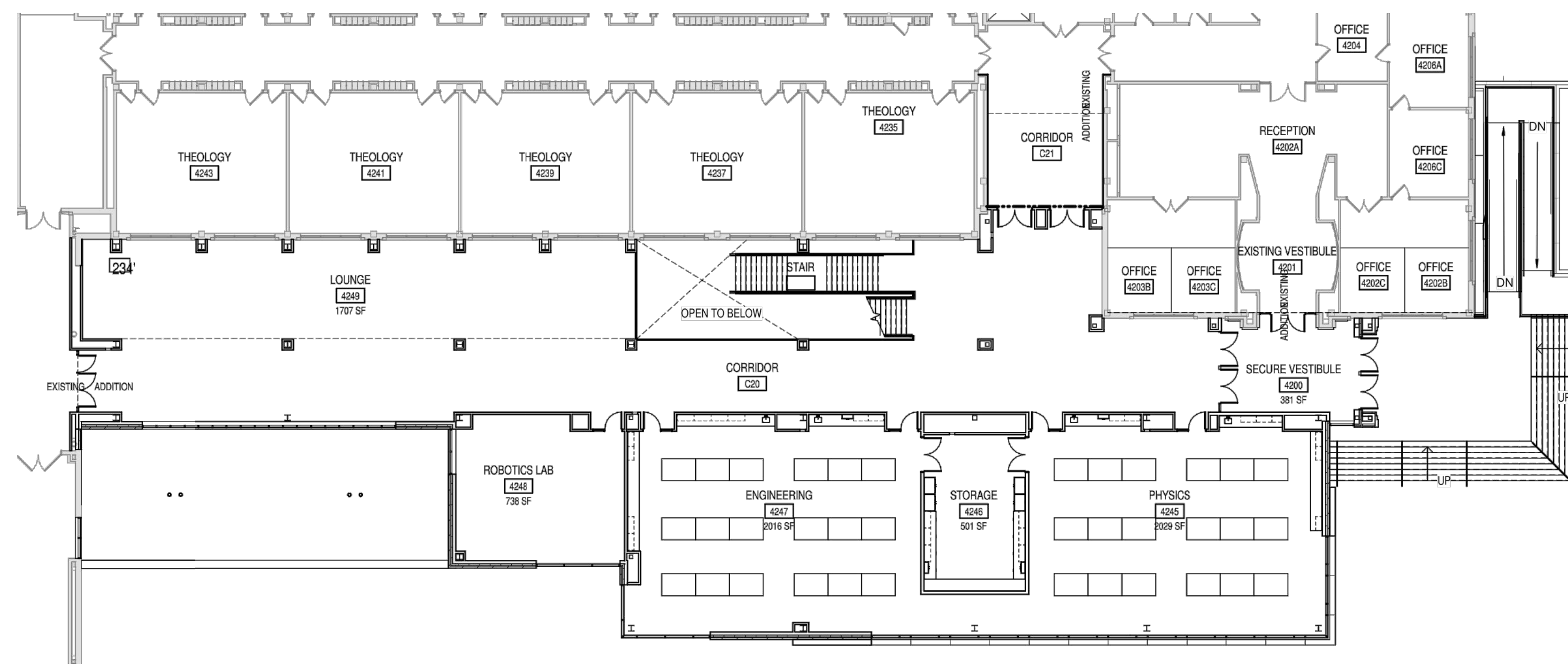
1 A102 FIRST FLOOR LIFE SAFETY PLAN
